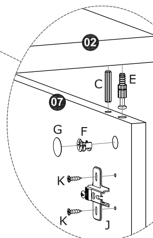
DETAIL 1
